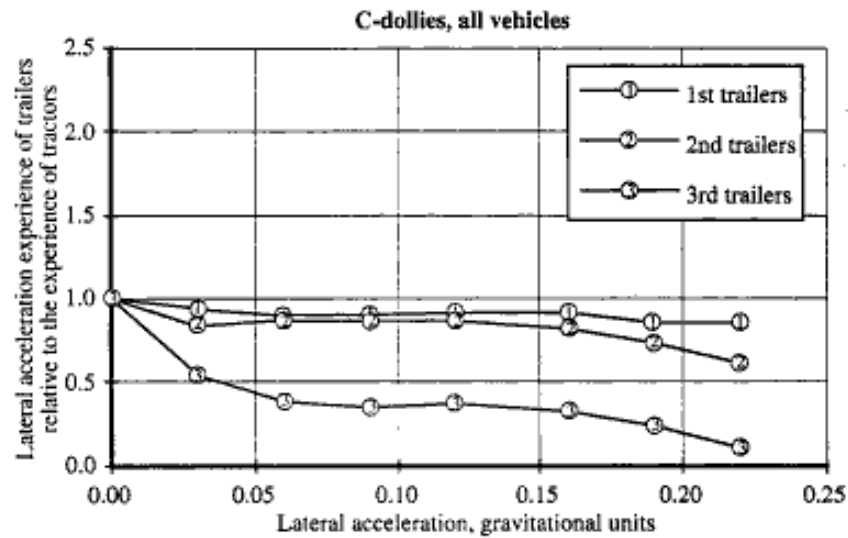
Figure 43. The lateral acceleration experience of all trailers relative to the lateral acceleration of tractors distinguished by trailer position and dolly type (speeds above 45 mph)
