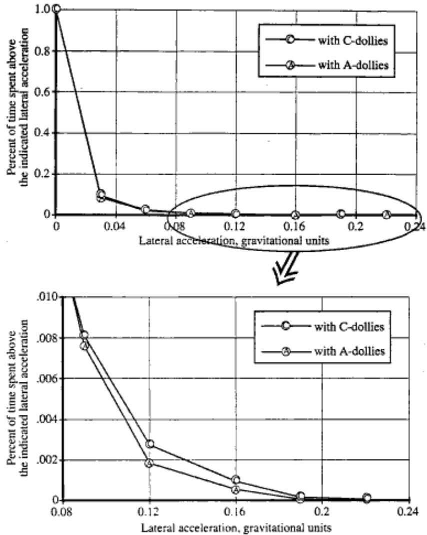
Figure 45. Comparison of the lateral acceleration experience of the tractors of triples when pulling A-dollies and C-dollies, respectively (speeds above 45 mph)
